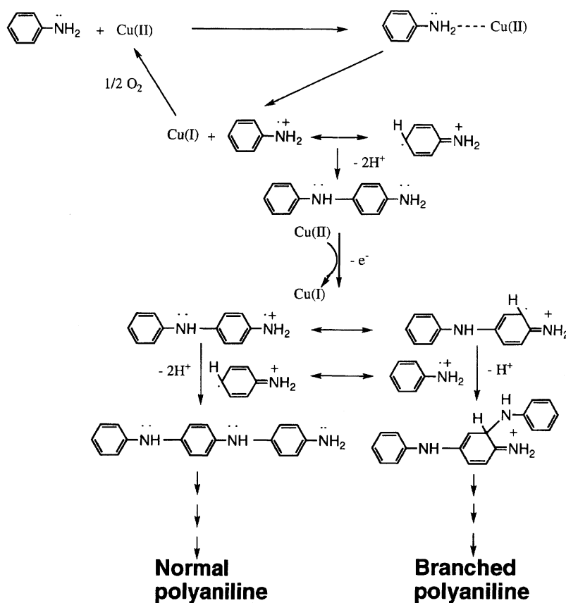
Scheme 2. Suggested mechanism of the polymerization of aniline.
